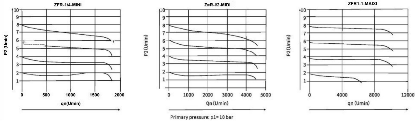
Standard flow rate qn as a function of the output pressure p2
